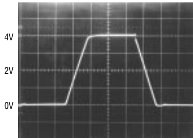
INPUT = 0V TO 4V PULSE
